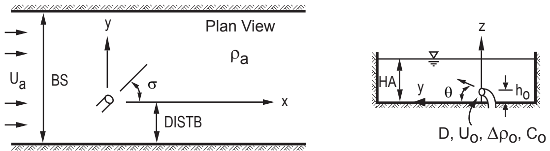
a) Definition Diagram CORMIX1 (Special case: HA = HD )
