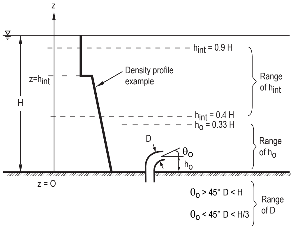
b) Limits of Applicability CORMIX1
