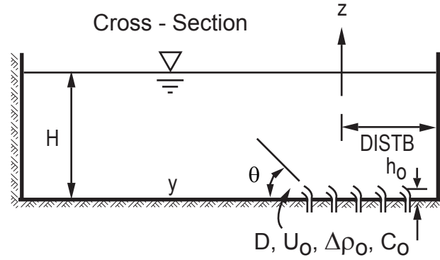
a) Definition Diagram CORMIX2
