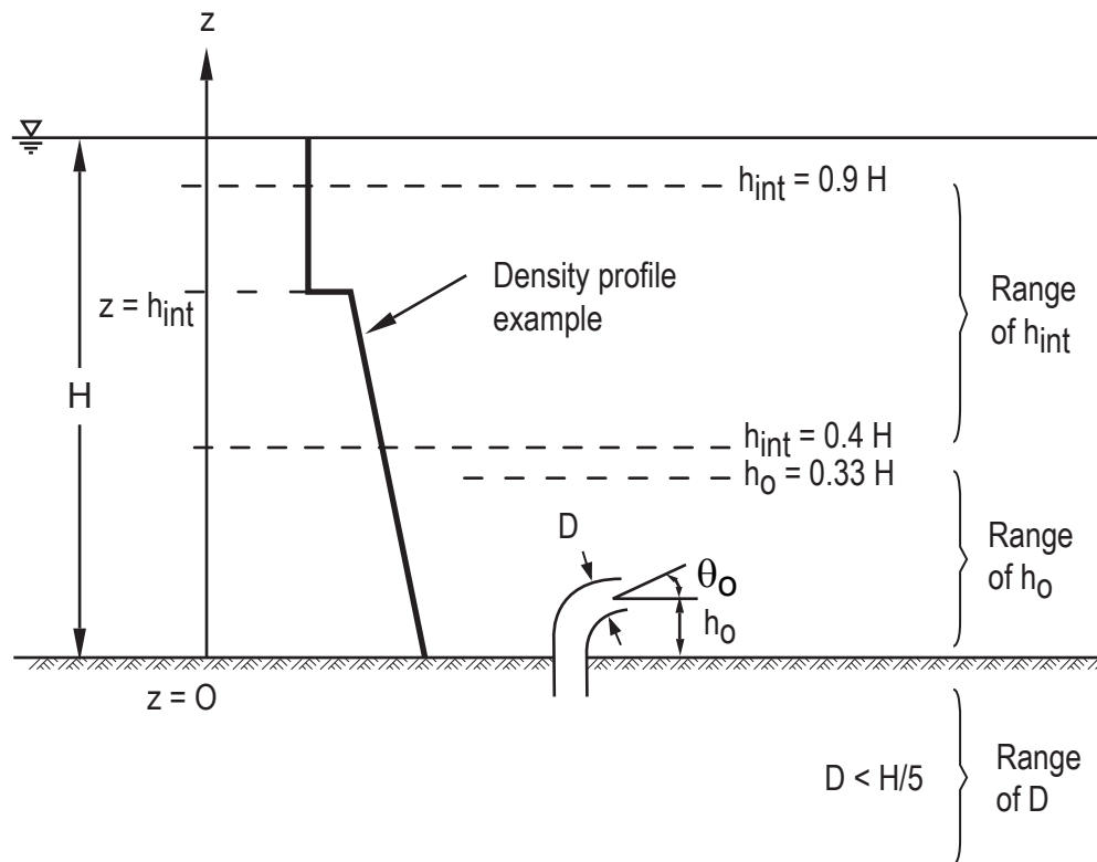
b) Limits of Applicability CORMIX 2
