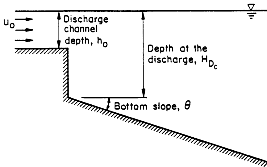
b) Cross-Section
