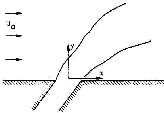
a) Discharge flush with bank
