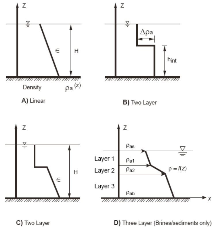
Figure 4.8 Different approximations for representing ambient density stratification.
