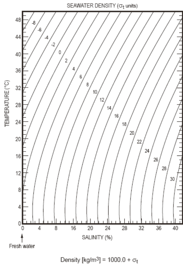
Figure 4.7 Diagram for density of seawater as a function of temperature and salinity
